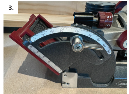
3. Set flip stop to desired angle and use the spacer plate if necessary. *Or use stop square for long point referencing
